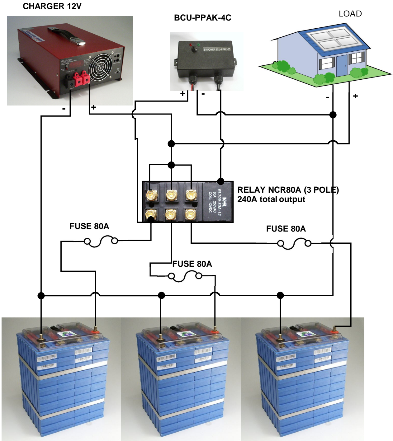
EV POWER PAK LFP BATTERY 12V 40-400Ah
